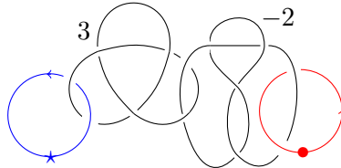
FIGURE 1. Surgery presentation of a toroidal cobordism
